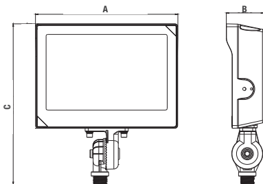
KNUCKLE MOUNT
