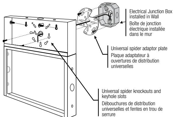
Fig. 2 Wall mount Montage mural
