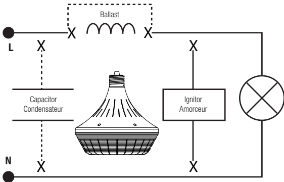
LED RETROFIT LAMP WIRING DIAGRAM SCHEMA DE CÂBLAGE LAMPE DEL RETROFIT
